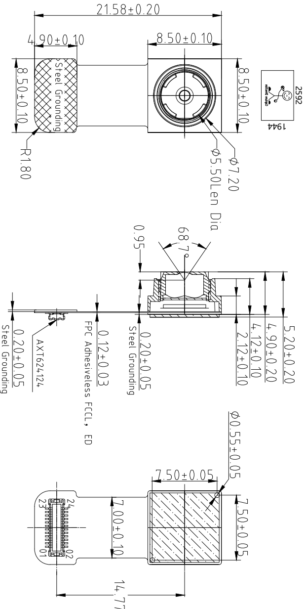
TOP VIEW
